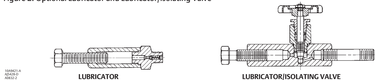
Figure 2. Optional Lubricator and Lubricator/Isolating Valve
